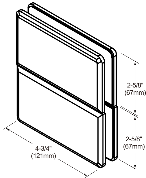
Senior Kara Code NO. SKPH2 Glass to Glass Hinge
